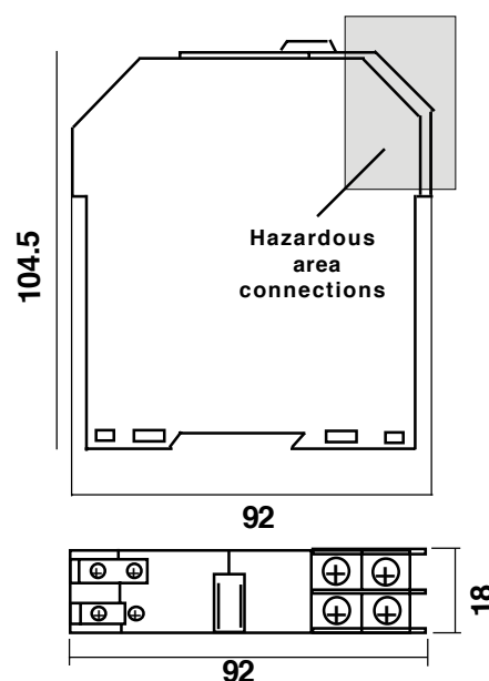
Housing Dimensions
